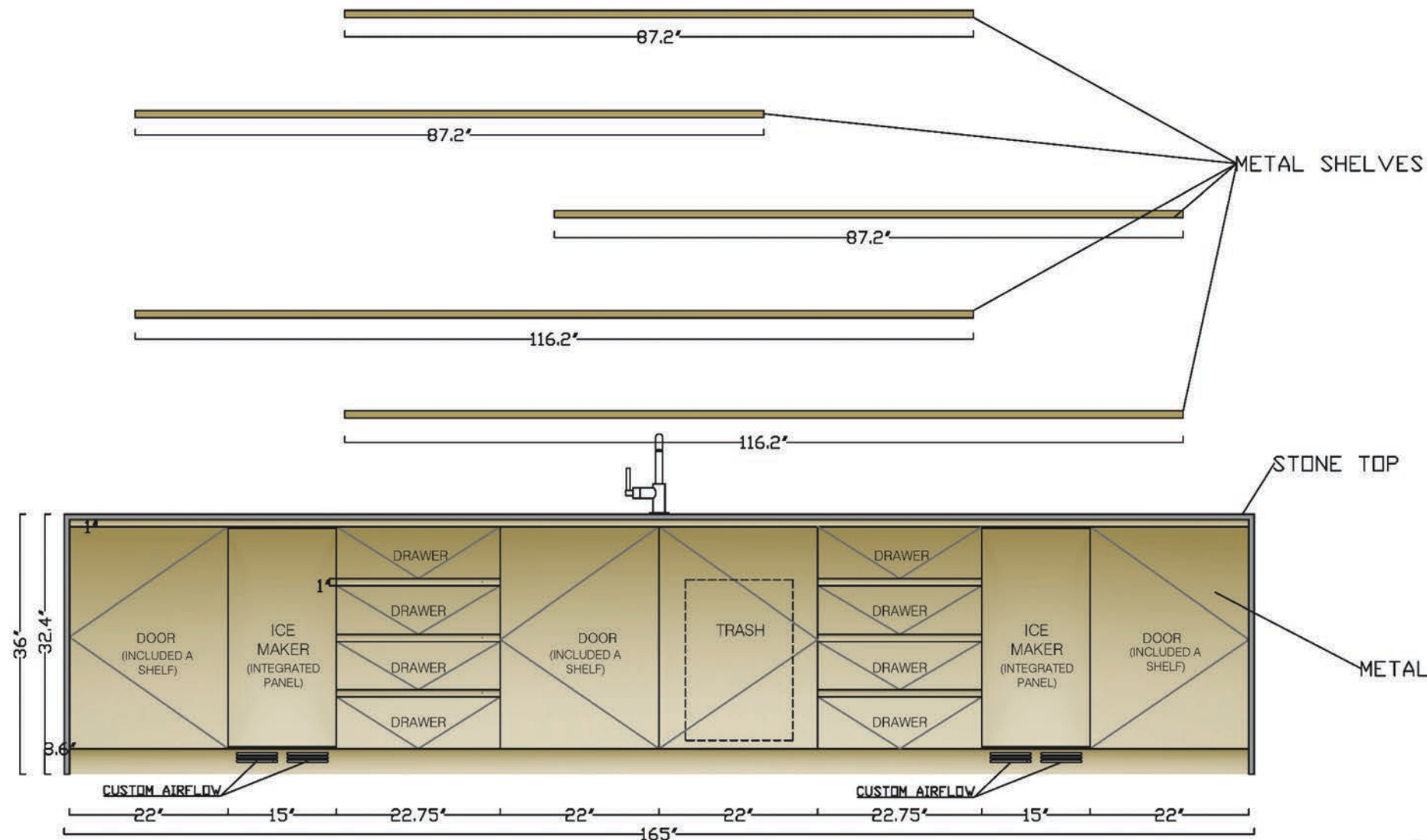
BAR FRONTAL VIEW
