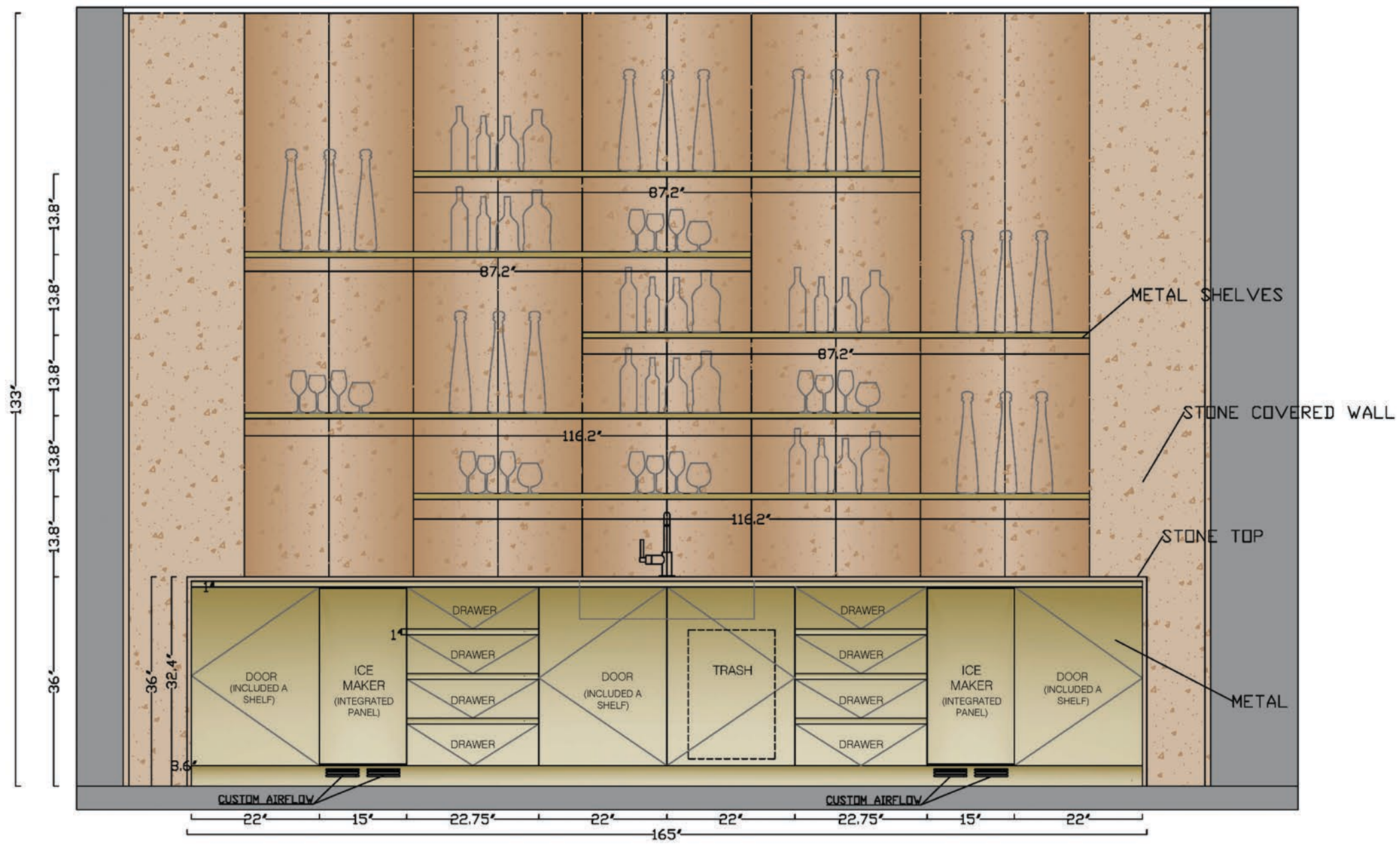
BAR FRONTAL VIEW
