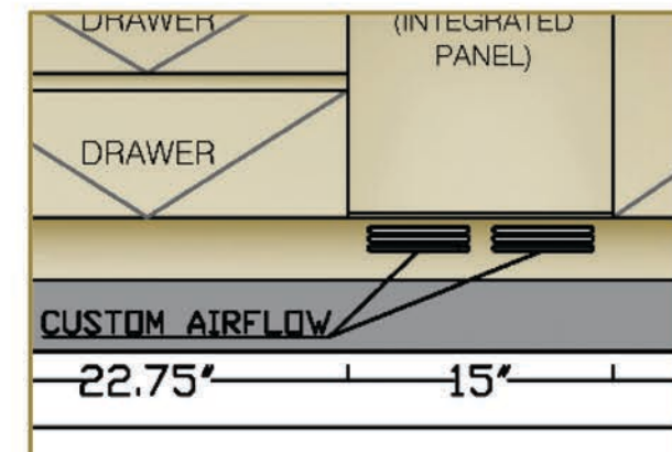
CUSTOM AIRFLOW DETAILS
