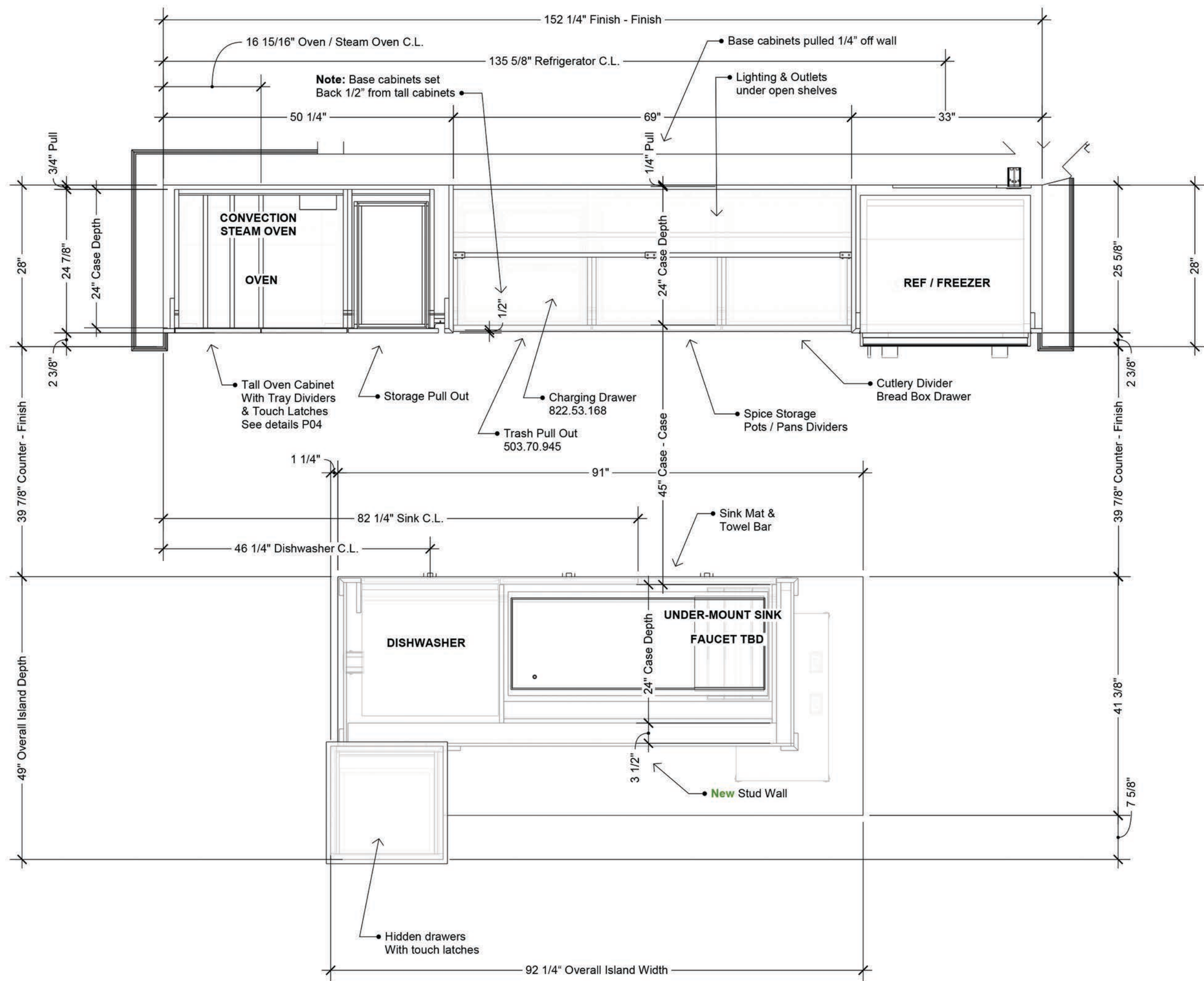
Kitchen Plan
