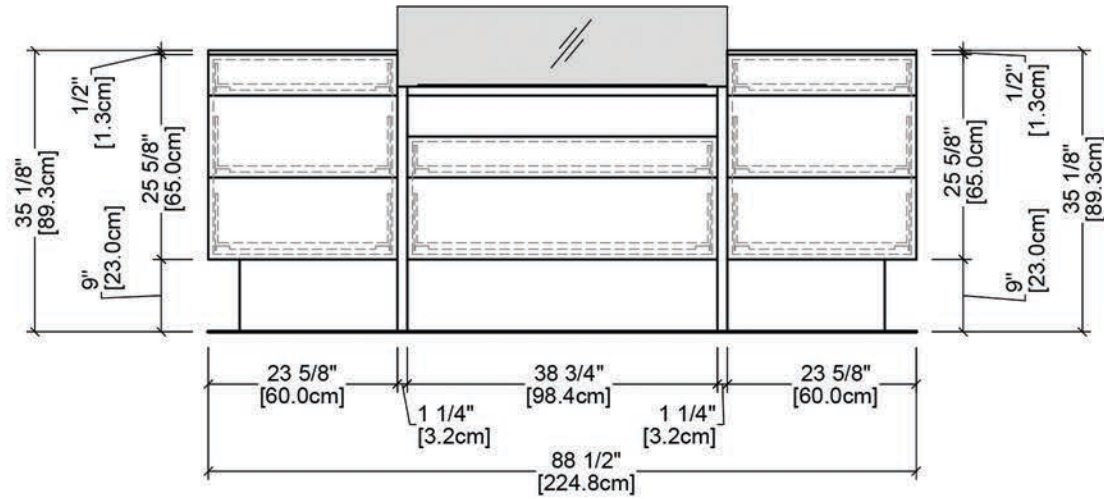
C ELEVATION 1/2"=1'-0"
