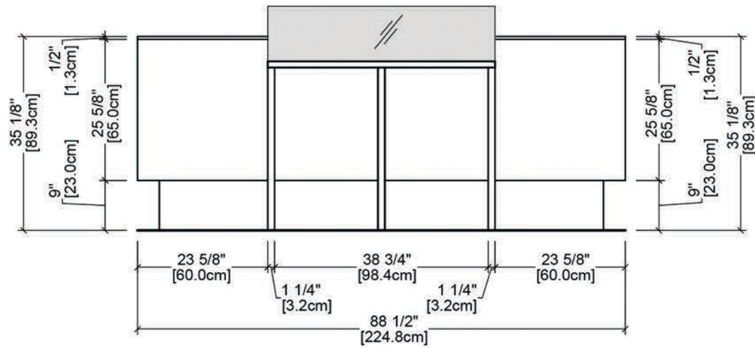
E ELEVATION 1/2"=1'-0"
