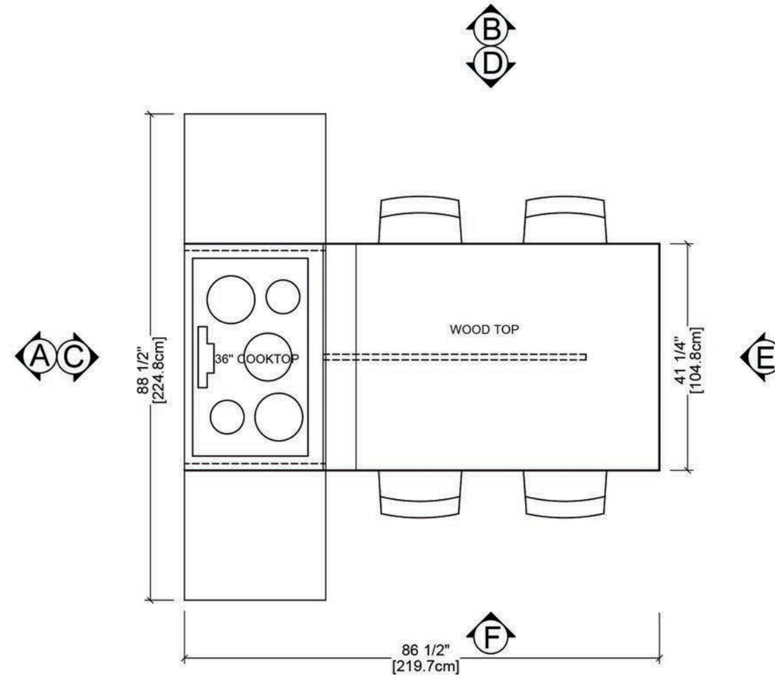
PLAN 1/2"=1'-0"
