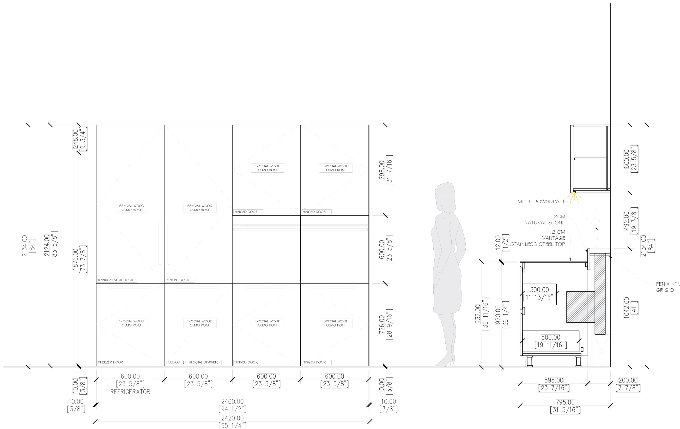
2 KITCHEN DISPLAY | ELEVATION
