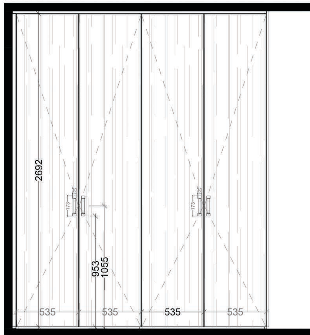
Elevation 4 - closed
