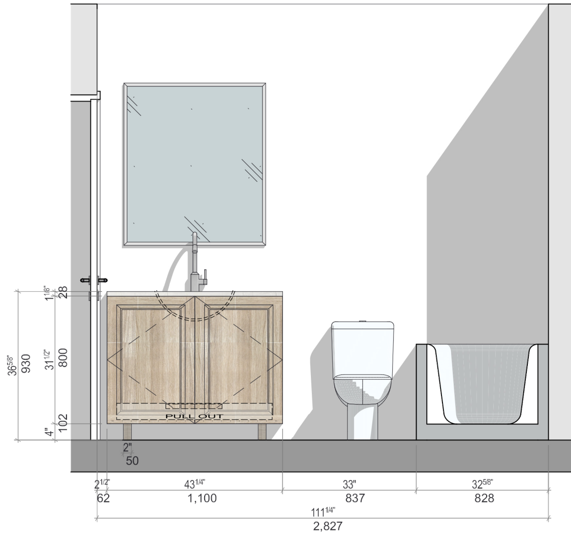
BHG-1 Elevation
