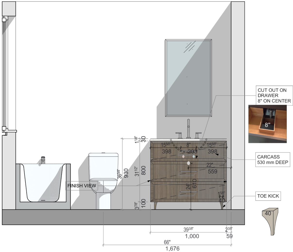
BH-3 Elevation
