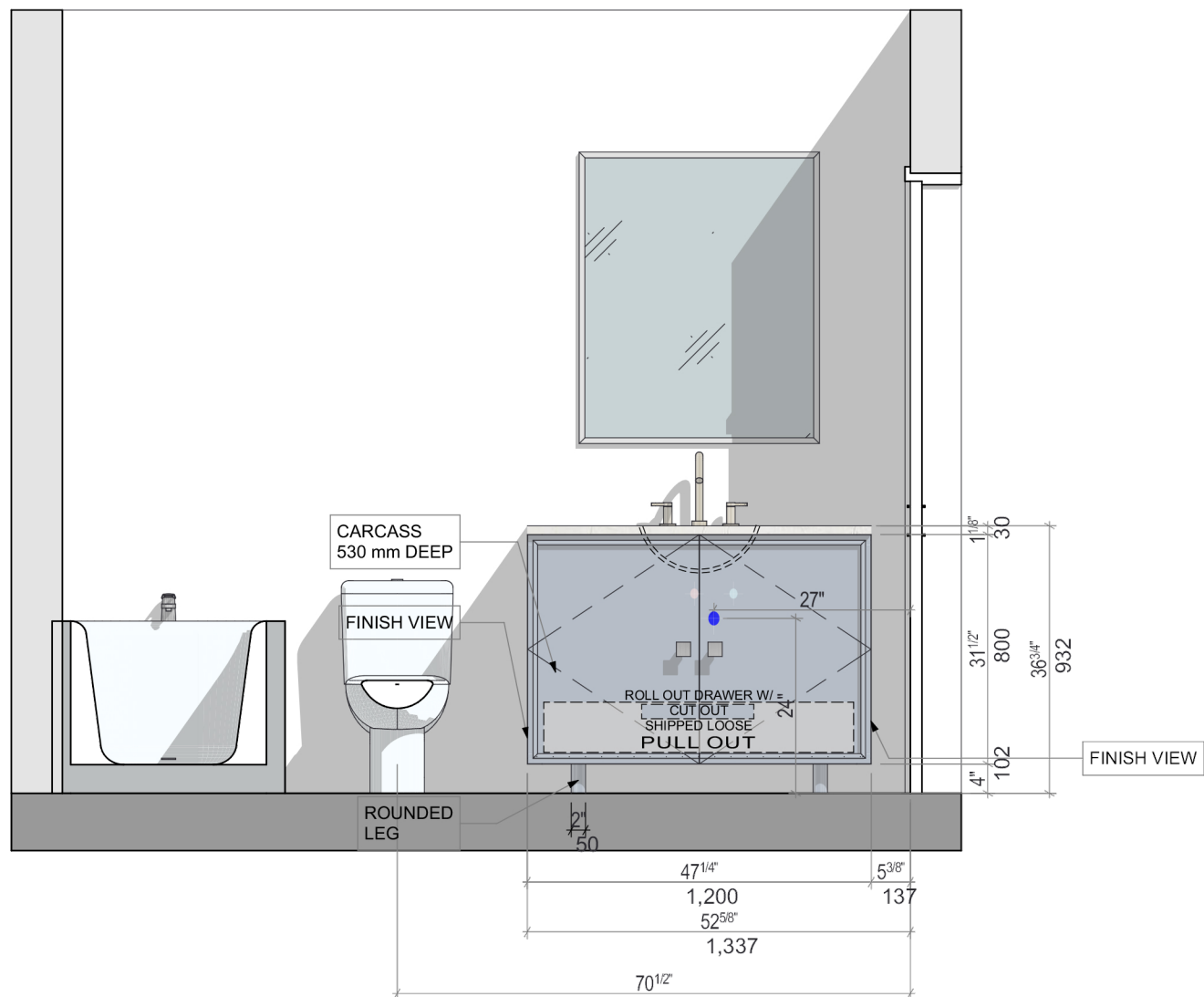
BH-6 Elevation
