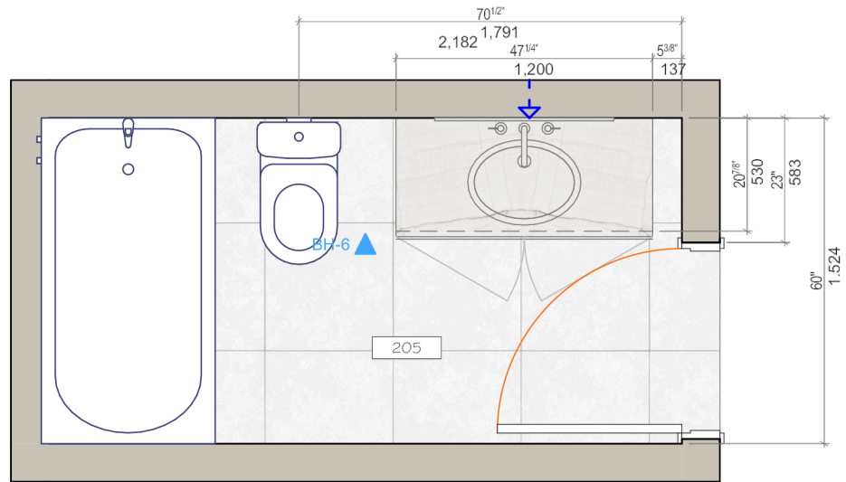
0. FLOOR PLAN
