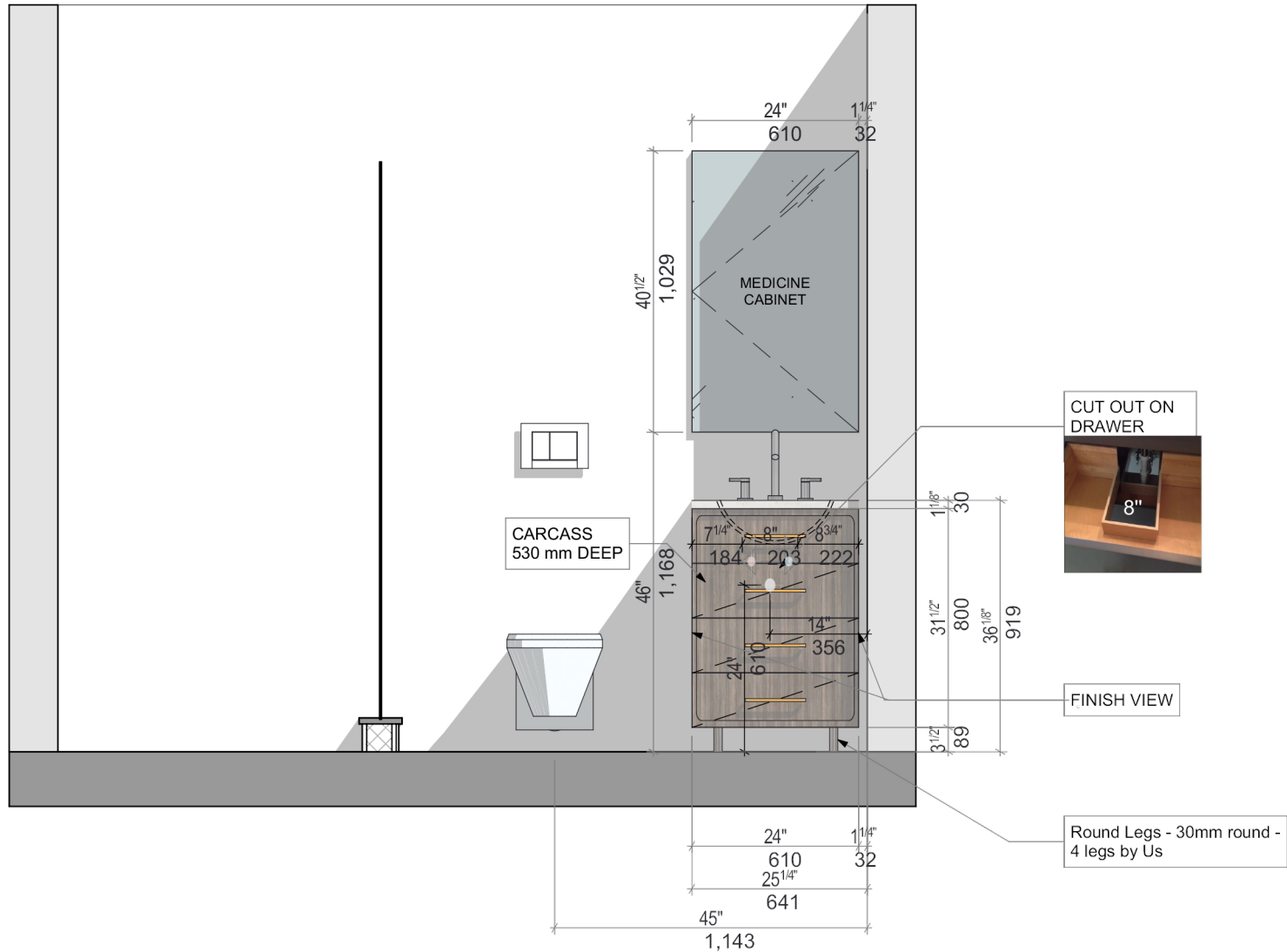
BH-4 Elevation
