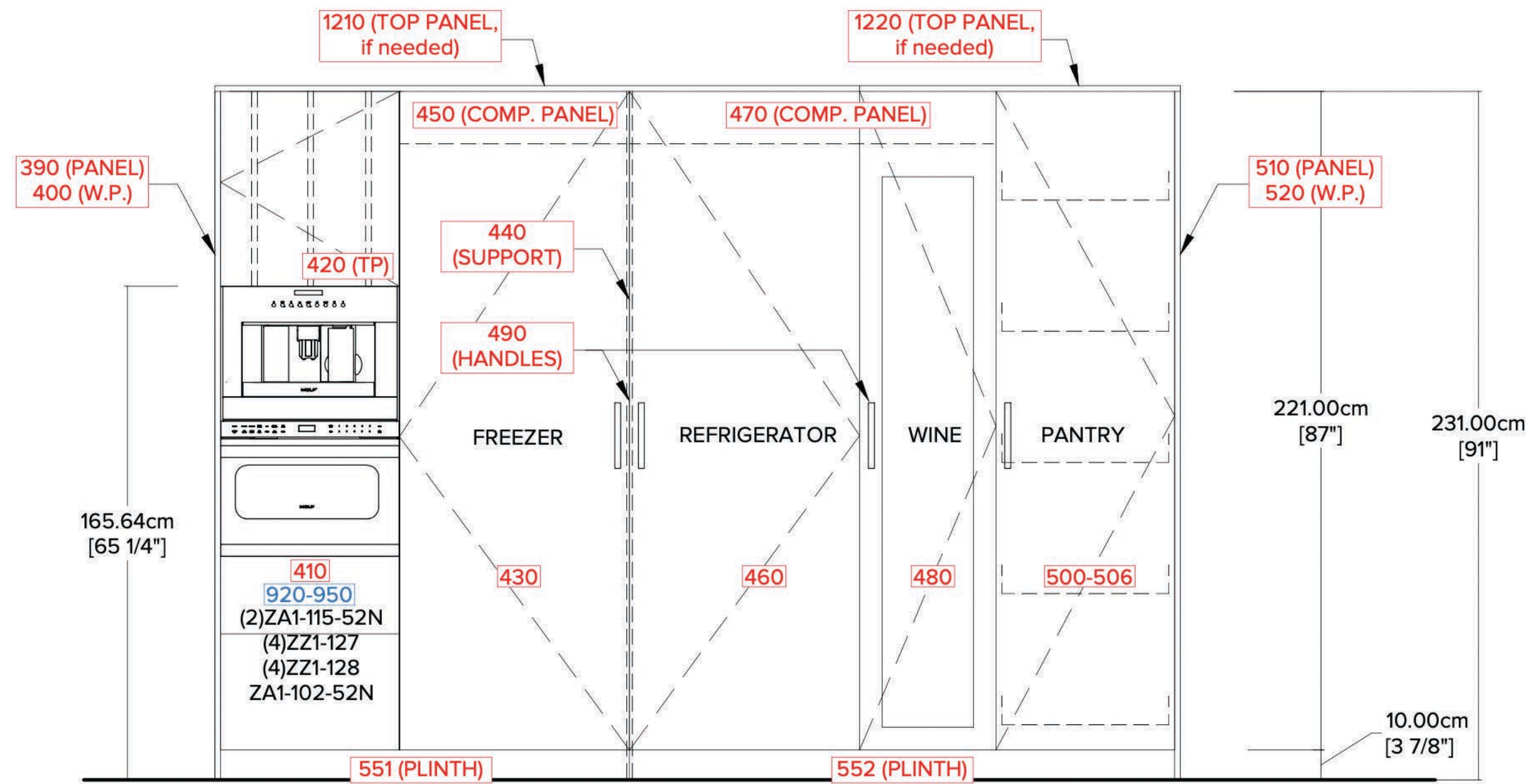
D ELEVATION
