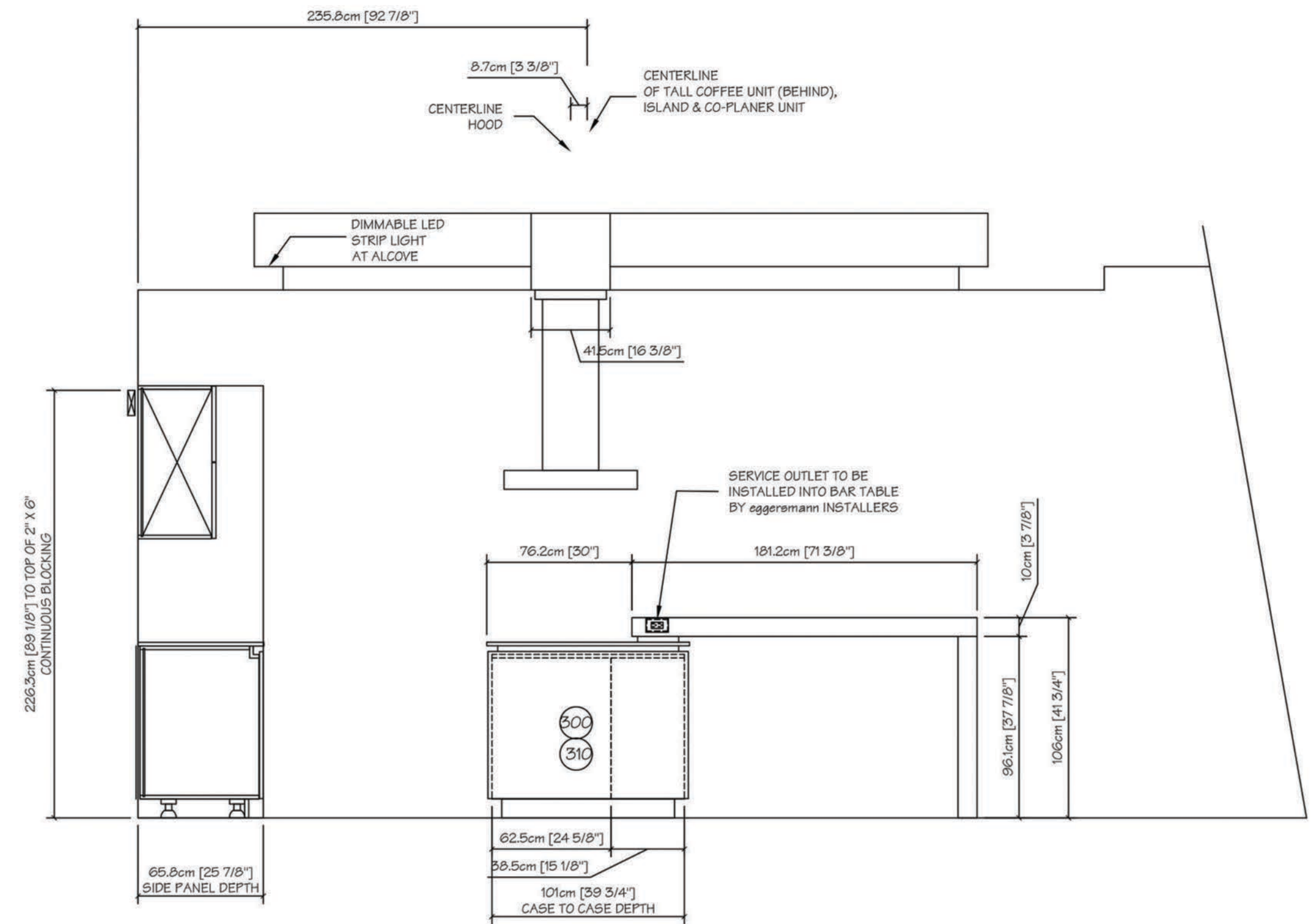
ELEVATION D
