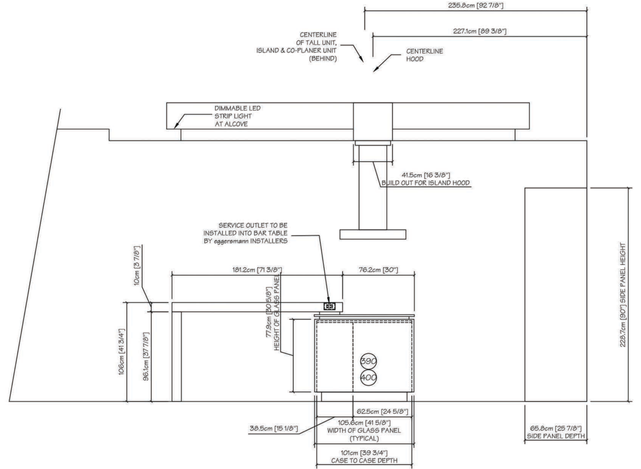
ELEVATION D
