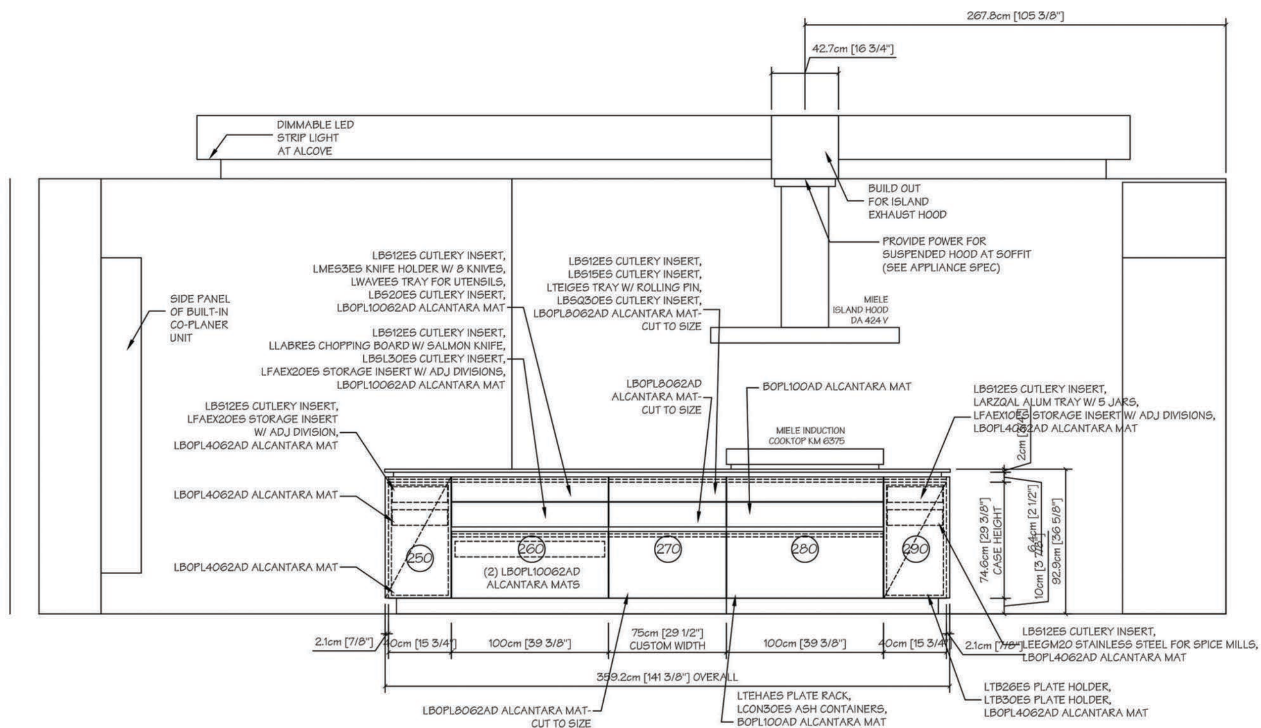
ELEVATION C
