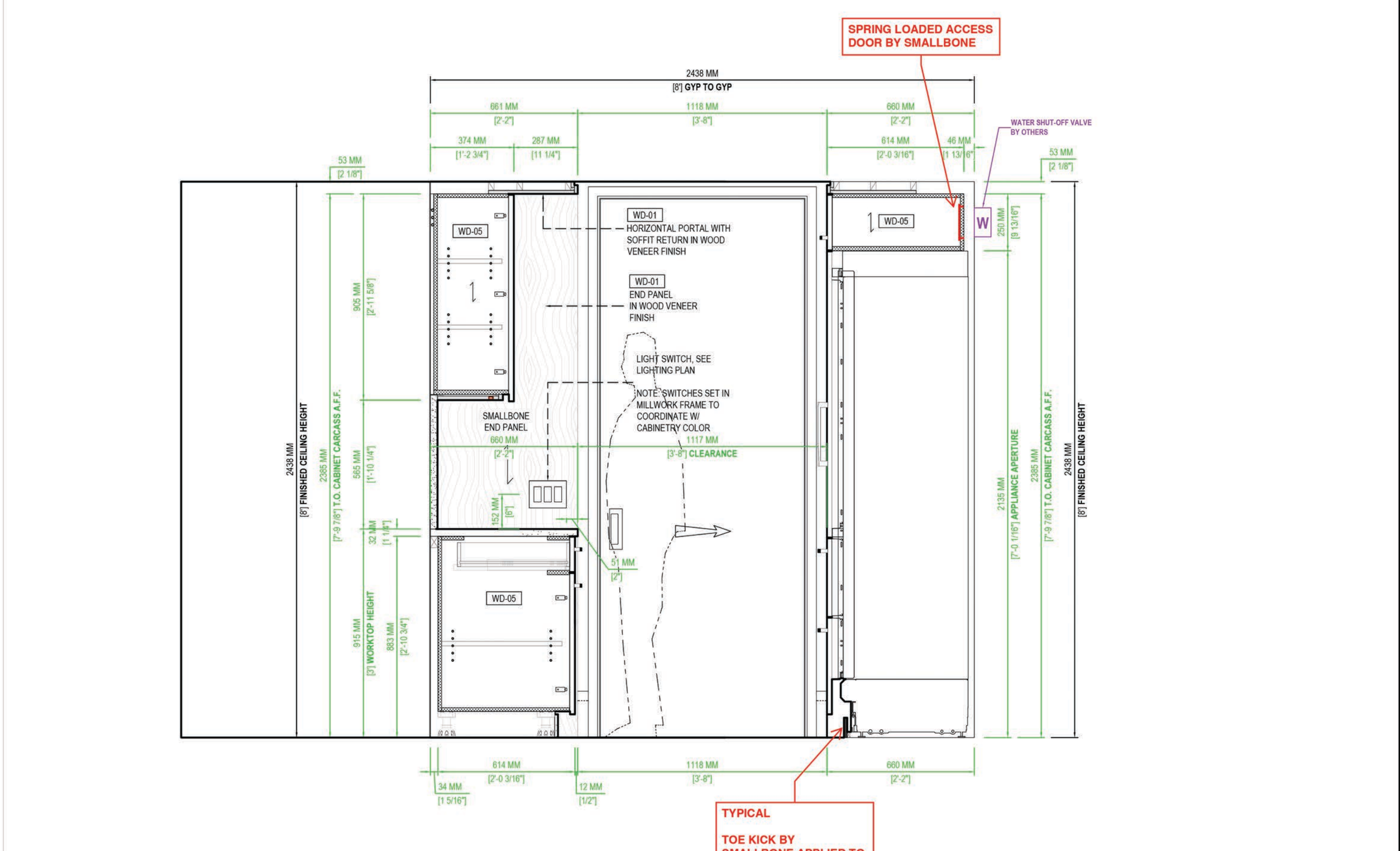
KITCHEN ELEVATION D TYPE 5
