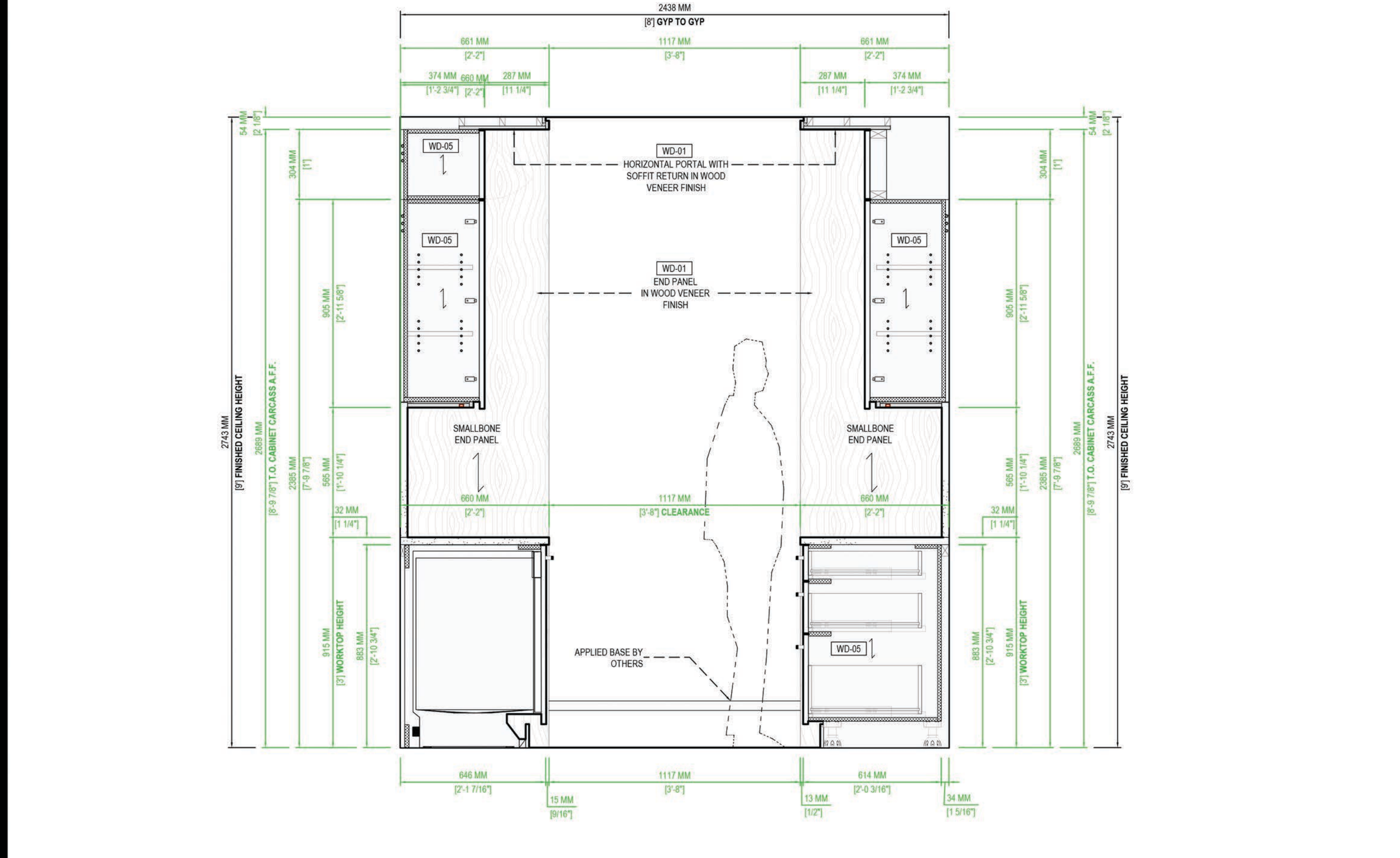
KITCHEN ELEVATION C TYPE 5
