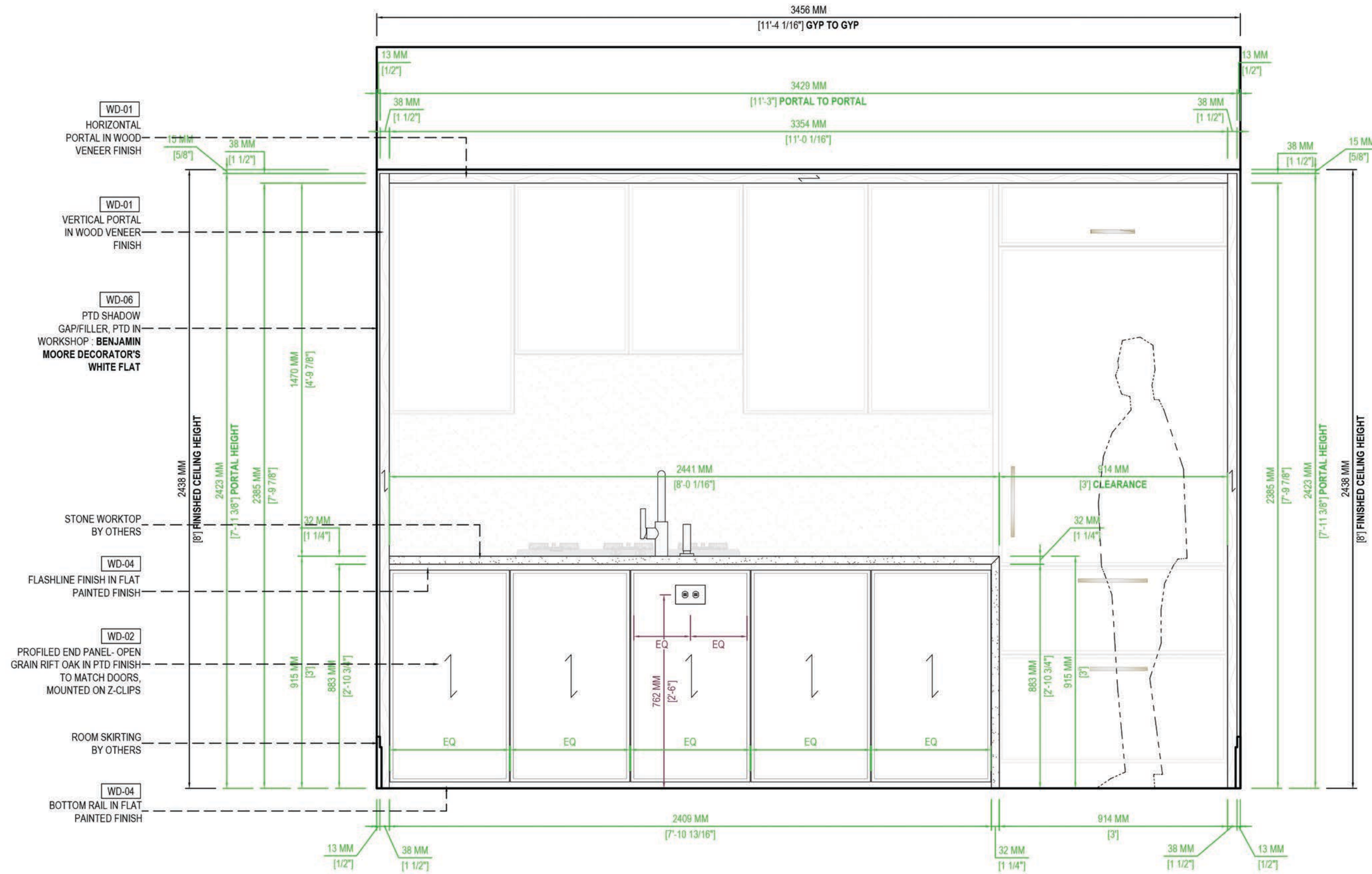
KITCHEN ELEVATION F TYPE 4
