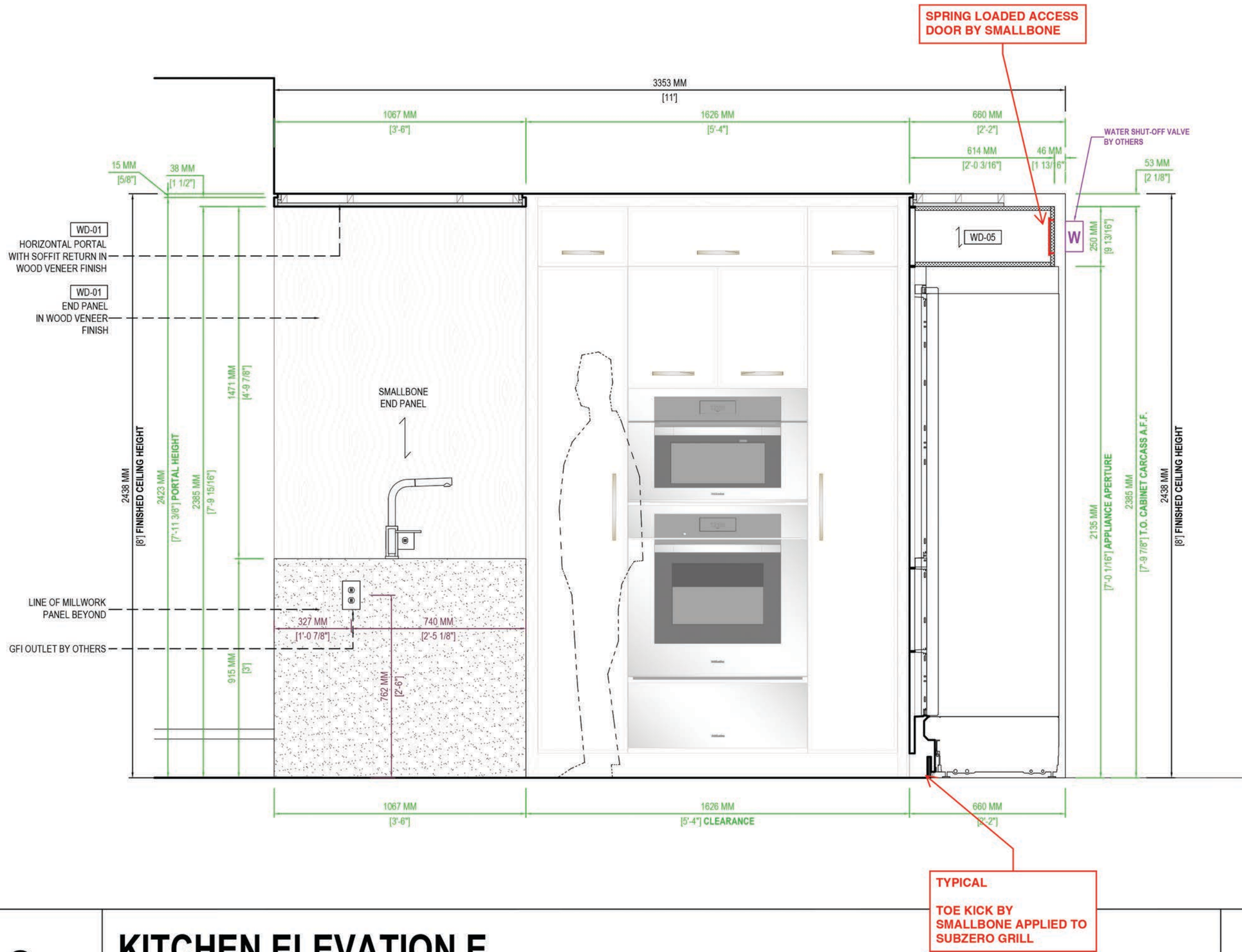
KITCHEN ELEVATION E TYPE 4
